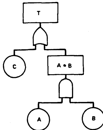
Figure VII-11. Fault Tree Equivalent of Figure VII-10
